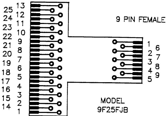
25 PIN FEMALE
