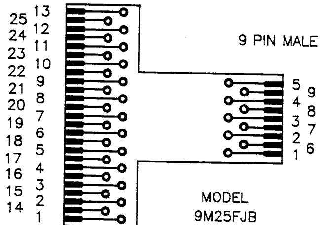
25 PIN FEMALE
