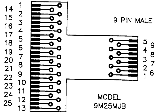
25 PIN MALE
