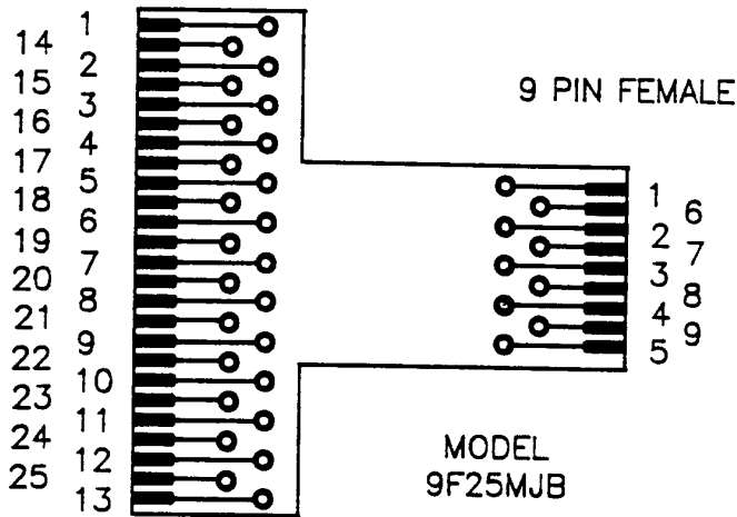
25 PIN MALE
