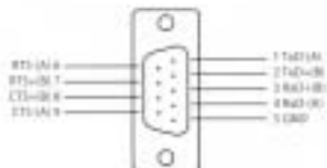
DB9 Male
