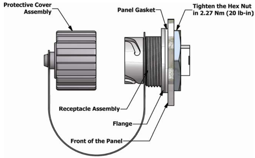
Figure 8-3: The Receptacle Panel Rear Mounting
