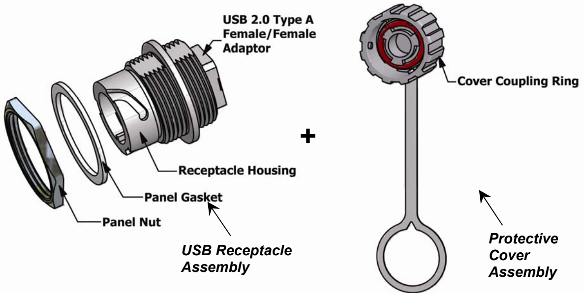
Figure 7-1: USB Receptacle + Protective Cover Assembly Kit
