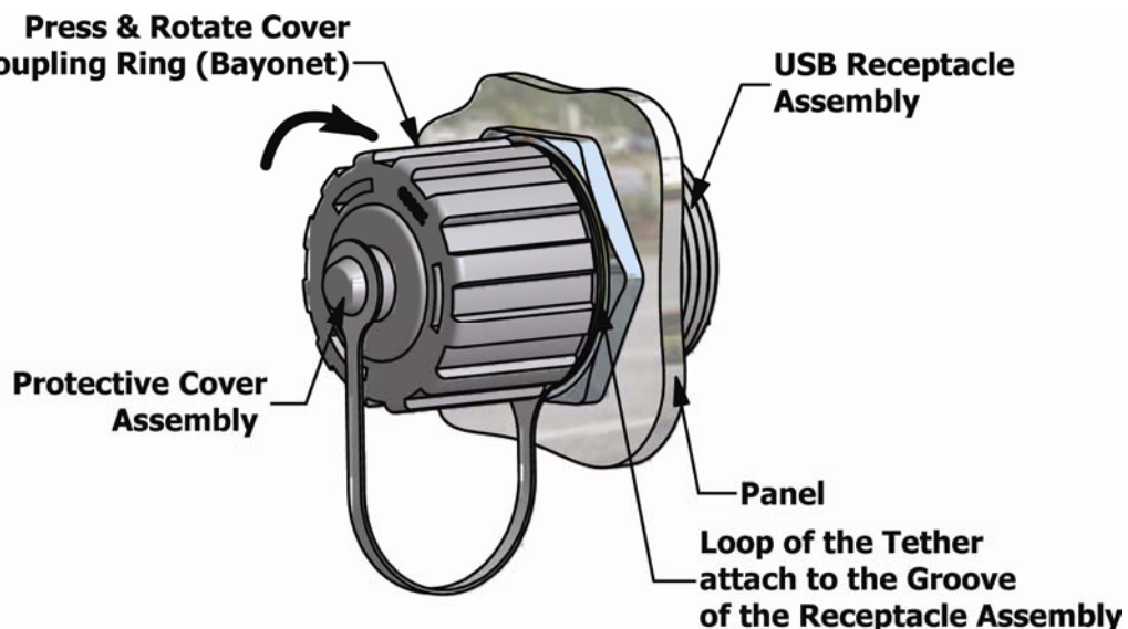
Figure 9-3: Cover Engagement (Bayonet Locking Style)
