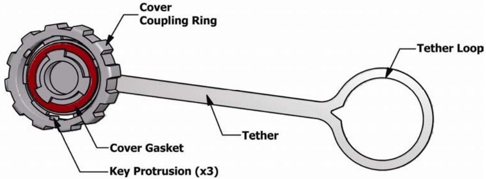
Figure 6-1: Protective Cover Assembly
