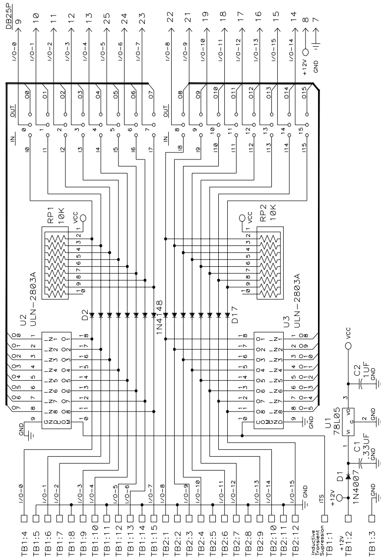
Figure C.10 - DBM16 Schematic
