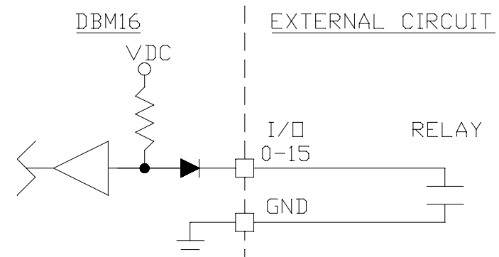
Figure C.5 - Isolated Mechanical Input
