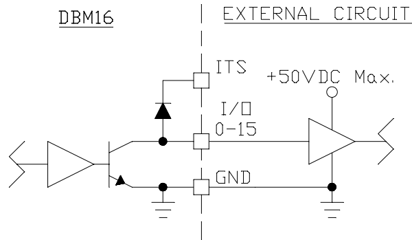
Figure C.7 - Solid State Output
