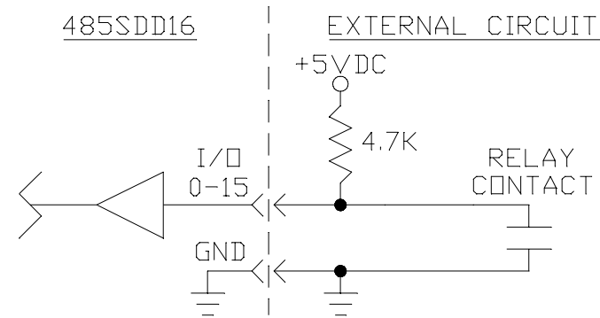
Figure 4.3 - Isolated Mechanical Input
