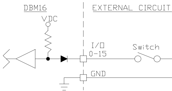
Figure C.3 - Switch Input
